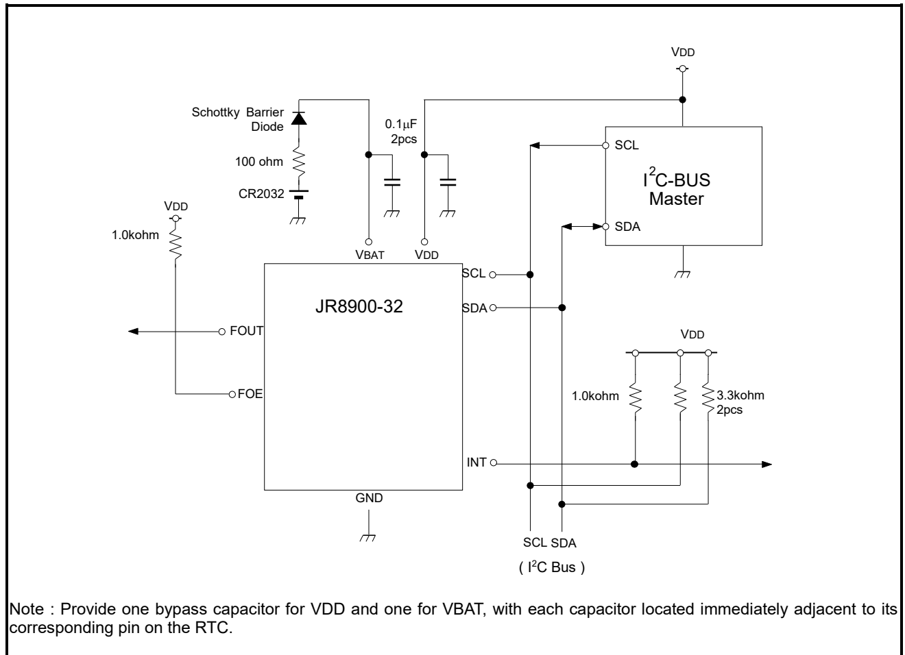
Figure 44 Connection example with Typical Microcontroller
