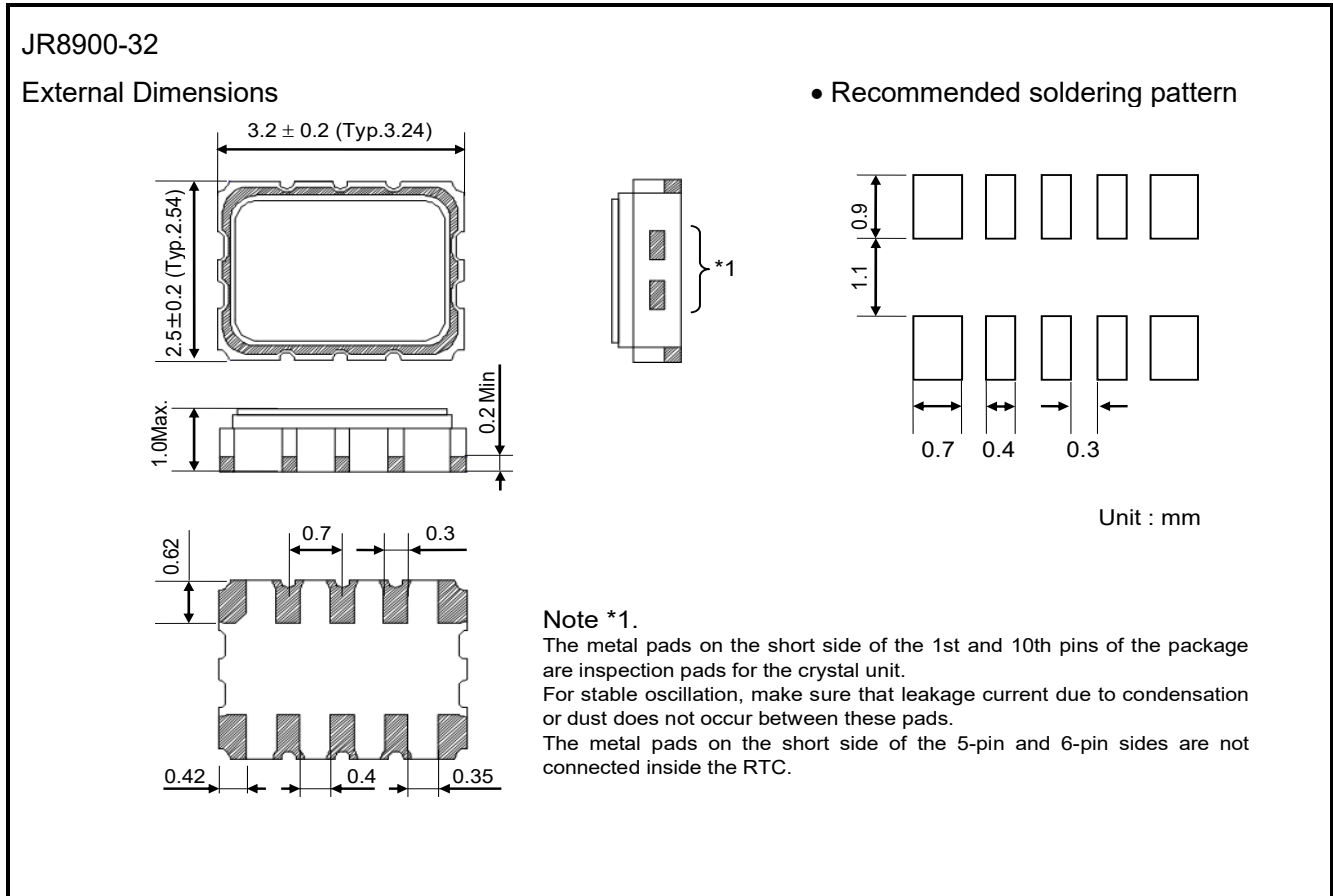
Figure 46 JR8900-32 package
