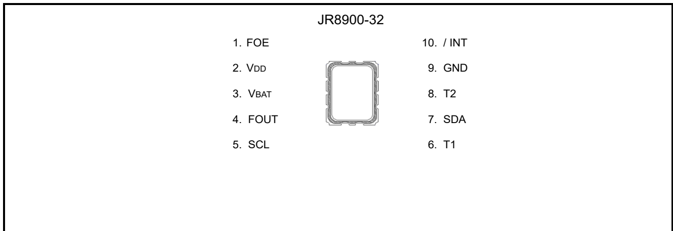
Figure 2 Terminal connections
