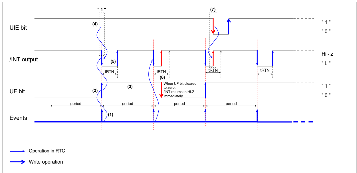
Figure 13 Time Update Interrupt Timing Chart.
