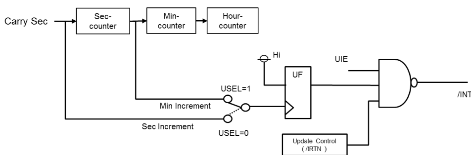
Figure 14 Time Update Interrupt Block Diagram
