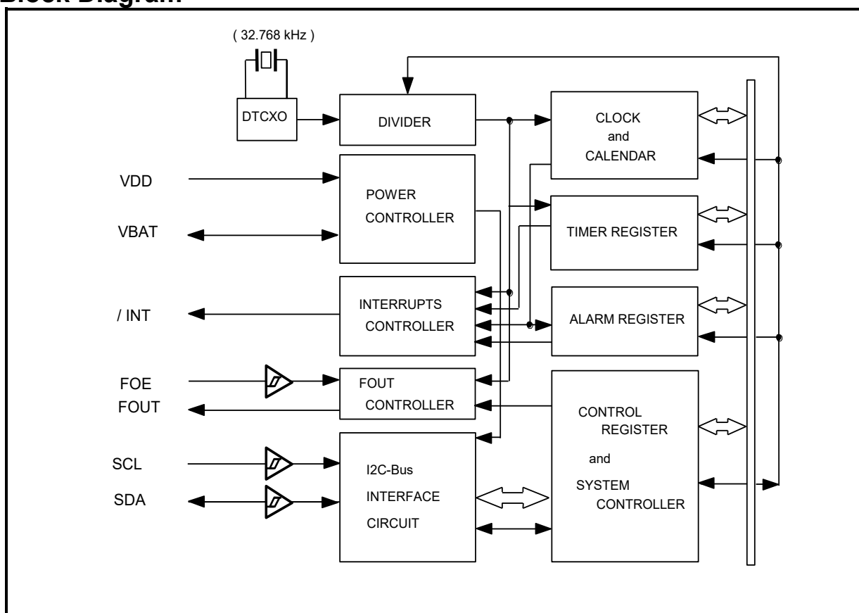
Figure 1 Block Diagram
