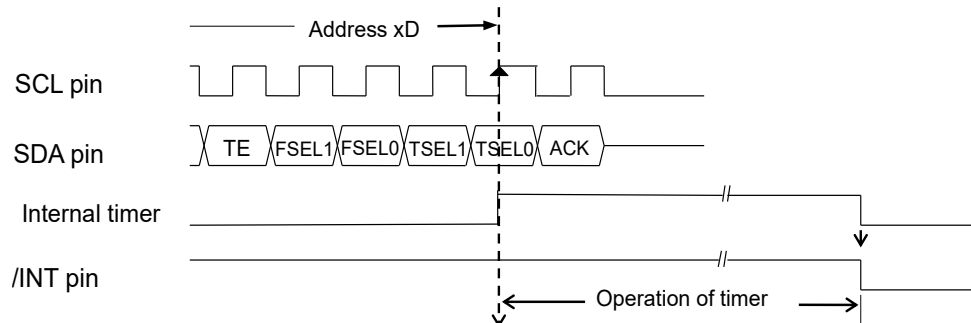
Figure 10 Fixed-cycle Timer start-timing.
