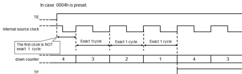
Figure 11 An error of first count down.
