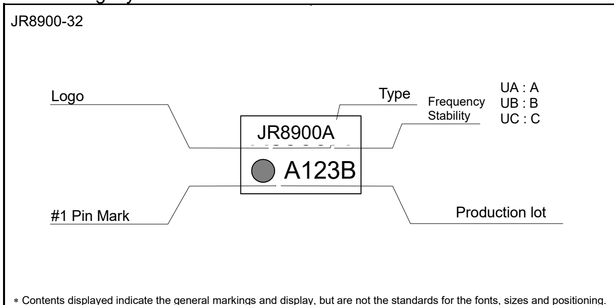
Figure 47JR8900-32 Marking layout
