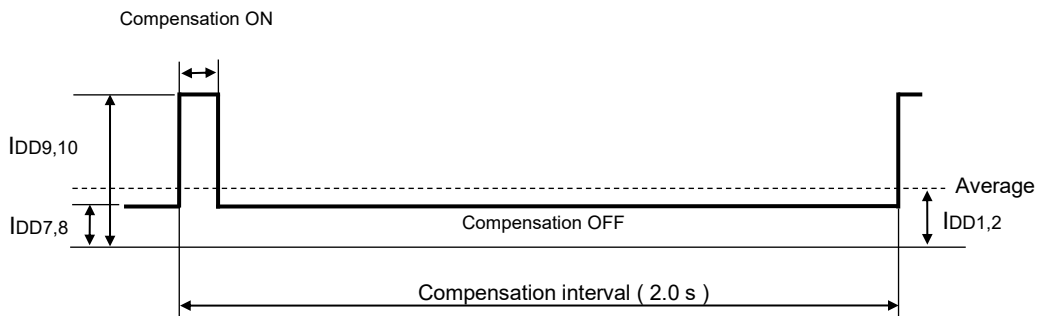
Figure 4 Definition for Current Consumption
