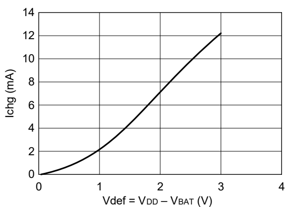
Figure 5.3 V_{BAT} Charging Characteristic ( V_{DD} = 3.0\text{ V} )
