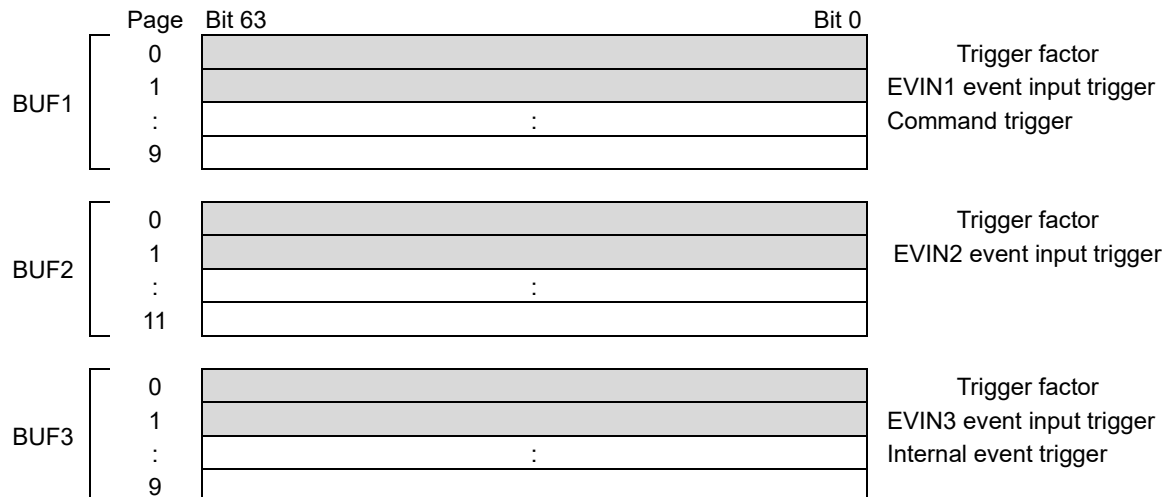
Figure 3.30 Time Stamp Buffer in Direct Mode (example when two data have been stored in each buffer)
