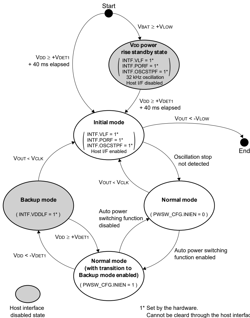
Figure 2.9 State Transition Diagram
