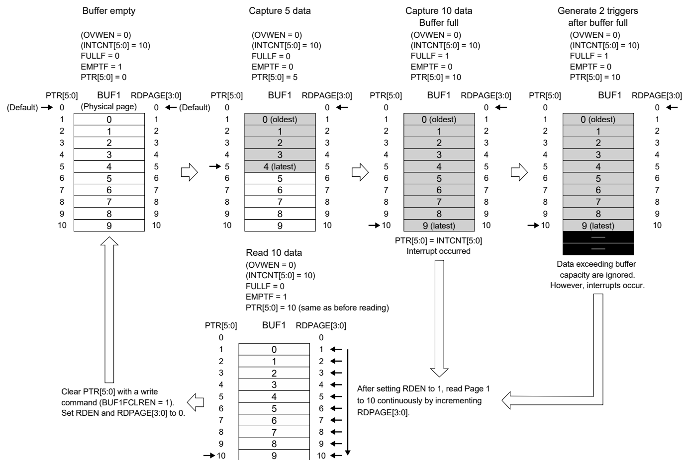
Figure 3.33 Time Stamp Capture Operations (Direct mode + Overwrite Inhibit mode)
