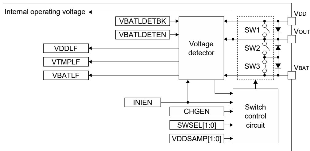
Figure 3.20 Auto Power Switching Circuit
