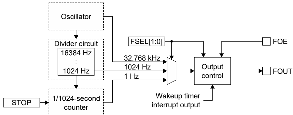
Figure 3.18 Configuration of FOUT Output Circuit
