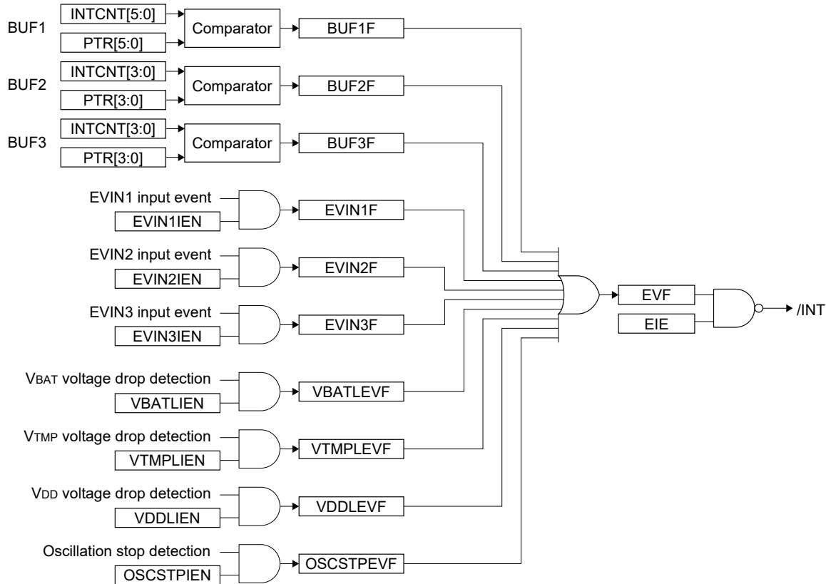
Figure 3.36 Configuration of Time Stamp Interrupt Circuit
