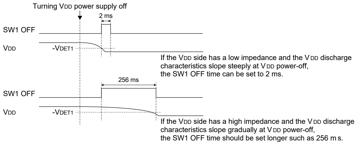
Figure 3.24 SW1 Intermittent Operation for Monitoring VDD Voltage
