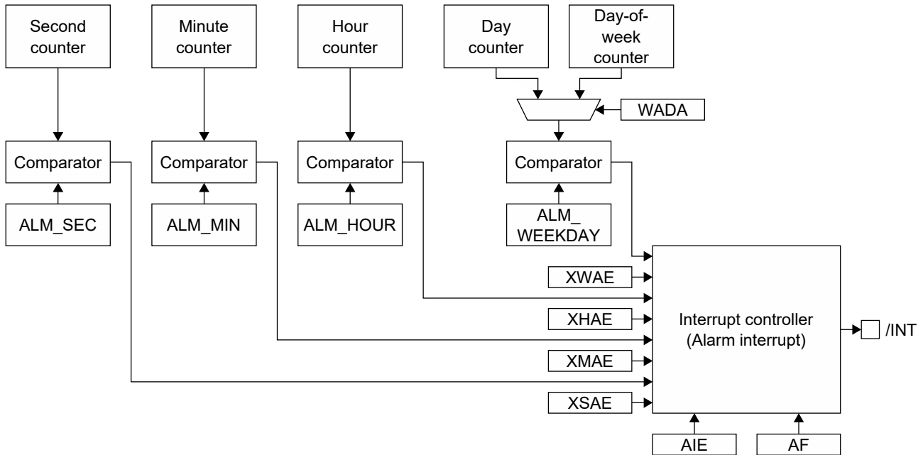
Figure 3.10 Configuration of Alarm Circuit
