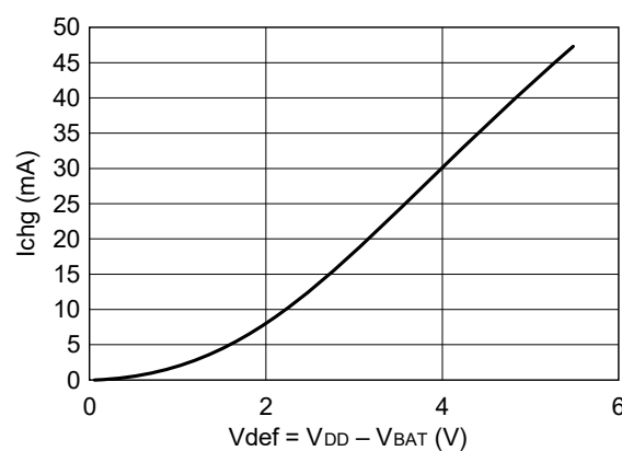
Figure 5.4 V_{BAT} Charging Characteristic ( V_{DD} = 5.5\text{ V} )
