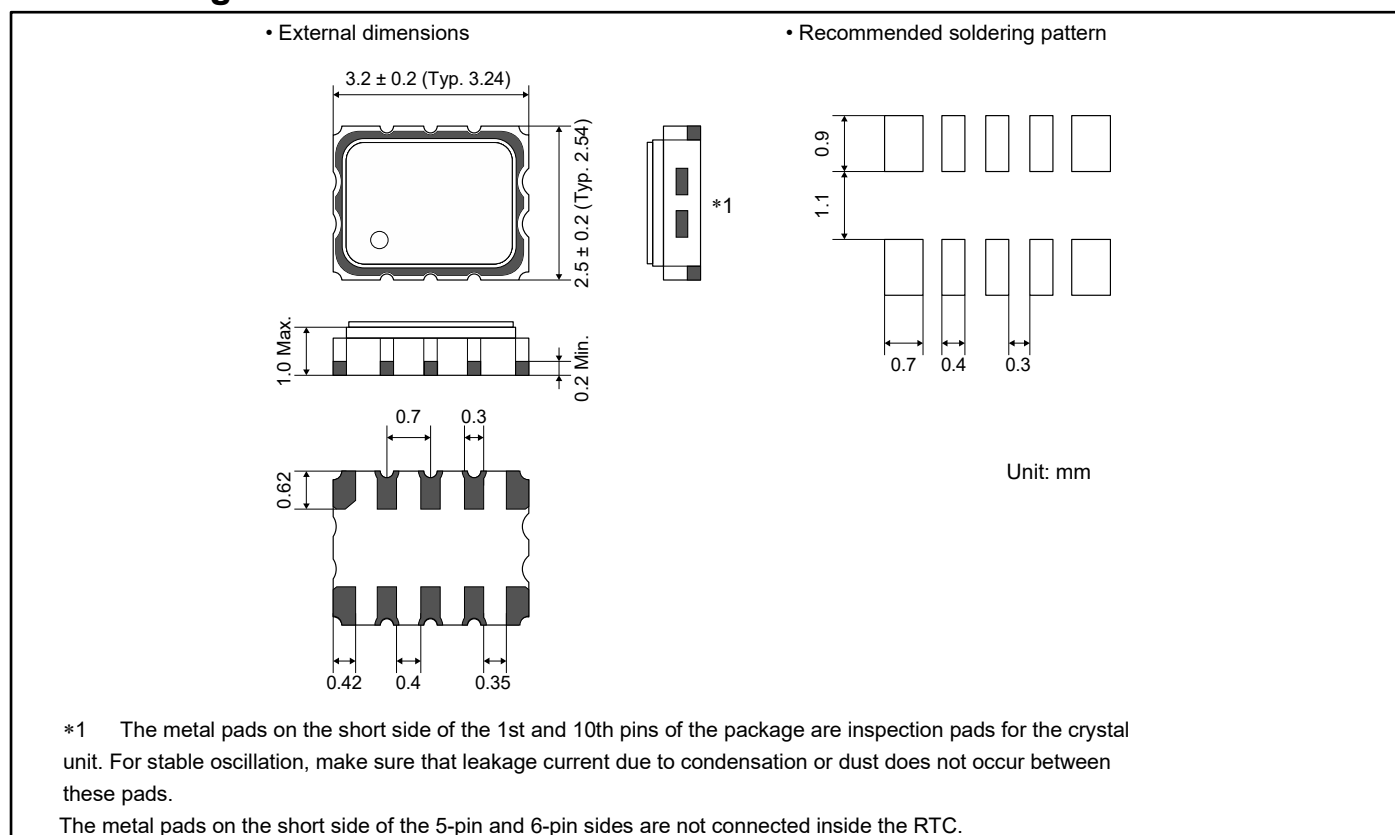
Figure 6.1 Package Dimensions
