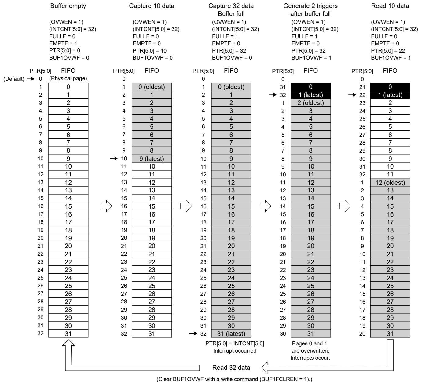
Figure 3.32 Time Stamp Capture Operations (FIFO mode + Overwrite mode)
