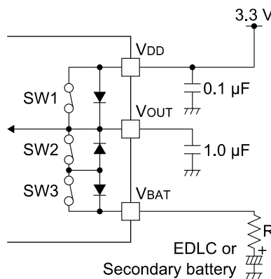
Figure 2.2 Power Supply Connection Example (1)
