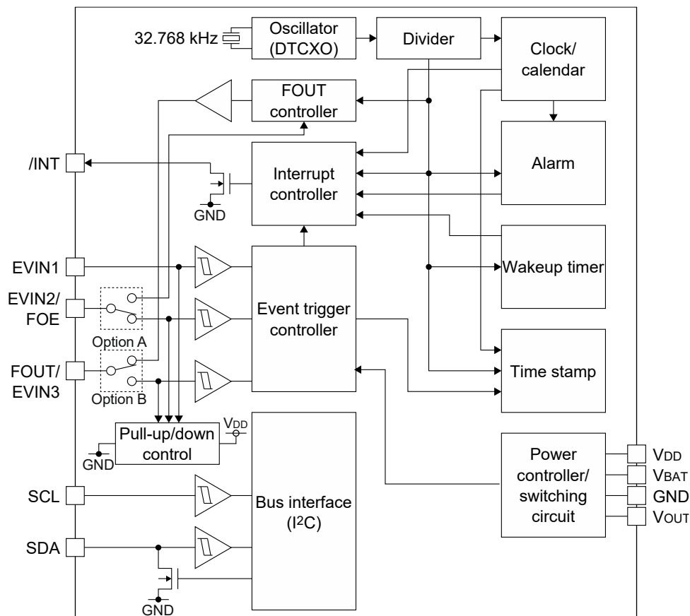
Figure 1.1 JR8901-32 Block Diagram
