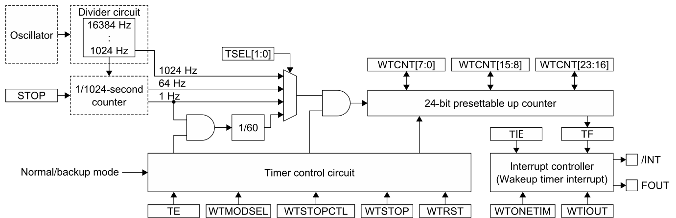
Figure 3.13 Configuration of Wakeup Timer
