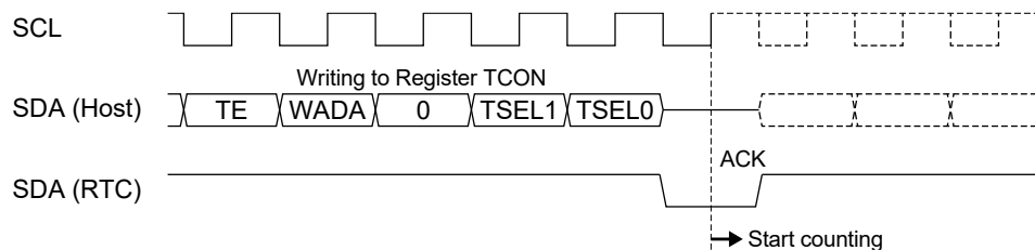
Figure 3.15 Wakeup Timer Count Start Timing
