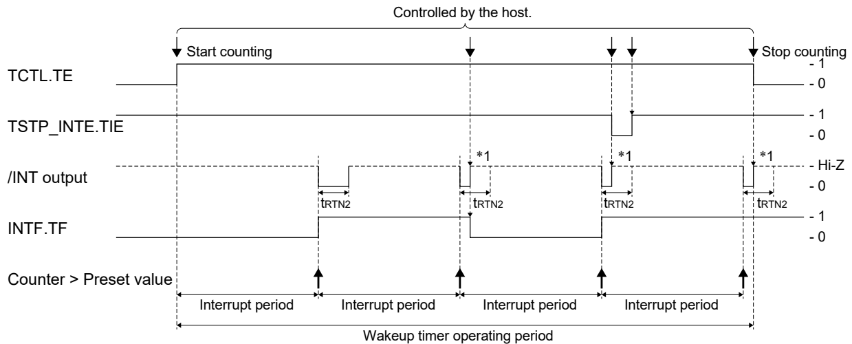
Figure 3.17 Wakeup Timer Interrupt Timing Chart
