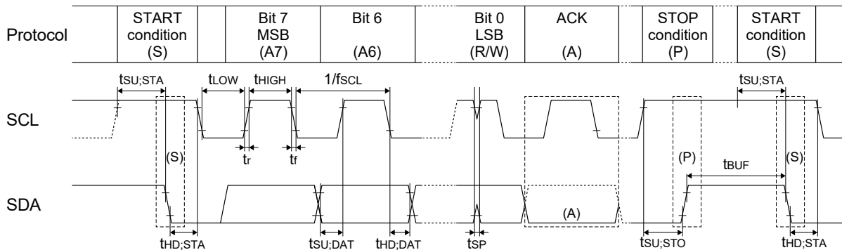
Figure 5.5 JR8901-32 AC Characteristics (I 2 C-Bus Timing Chart)
