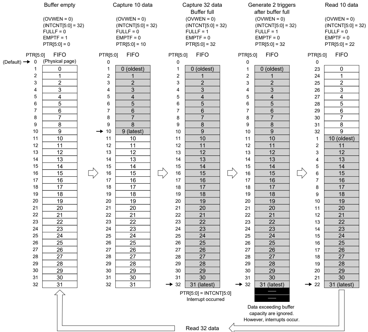
Figure 3.31 Time Stamp Capture Operations (FIFO mode + Overwrite Inhibit mode)
