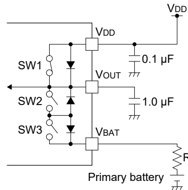
Figure 2.3 Power Supply Connection Example (2)
