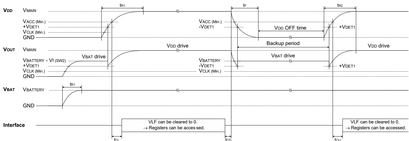
Figure 5.6 Power-On Sequence
