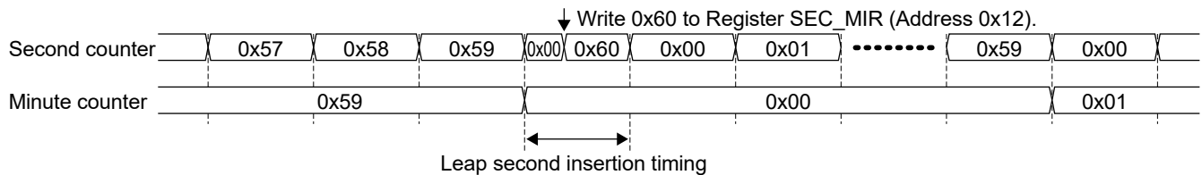
Figure 3.7 Leap Second Insertion Timing
