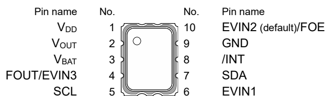
Figure 1.2 JR8901-32 Option EV/FO Pin Alignment Diagram
