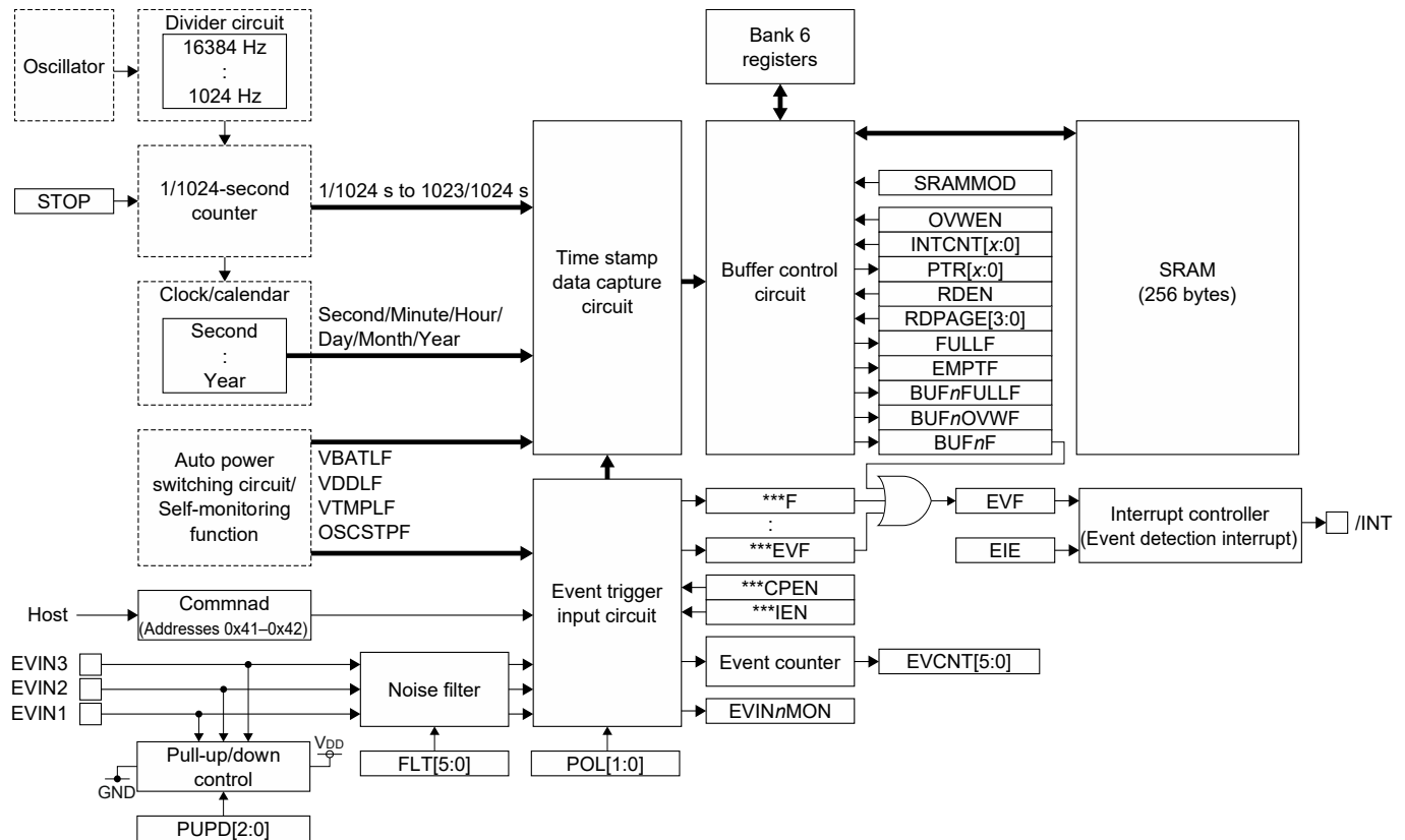
Figure 3.26 Configuration of Time Stamp Circuit
