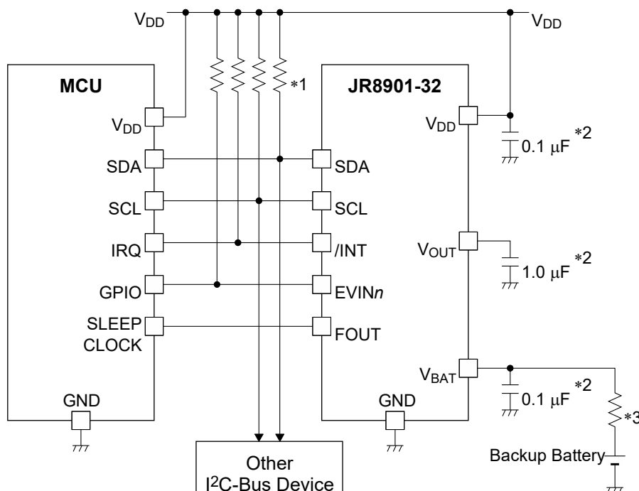
Figure 8.1 Sample Connection Diagram with a Typical MCU (JR8901-32)
