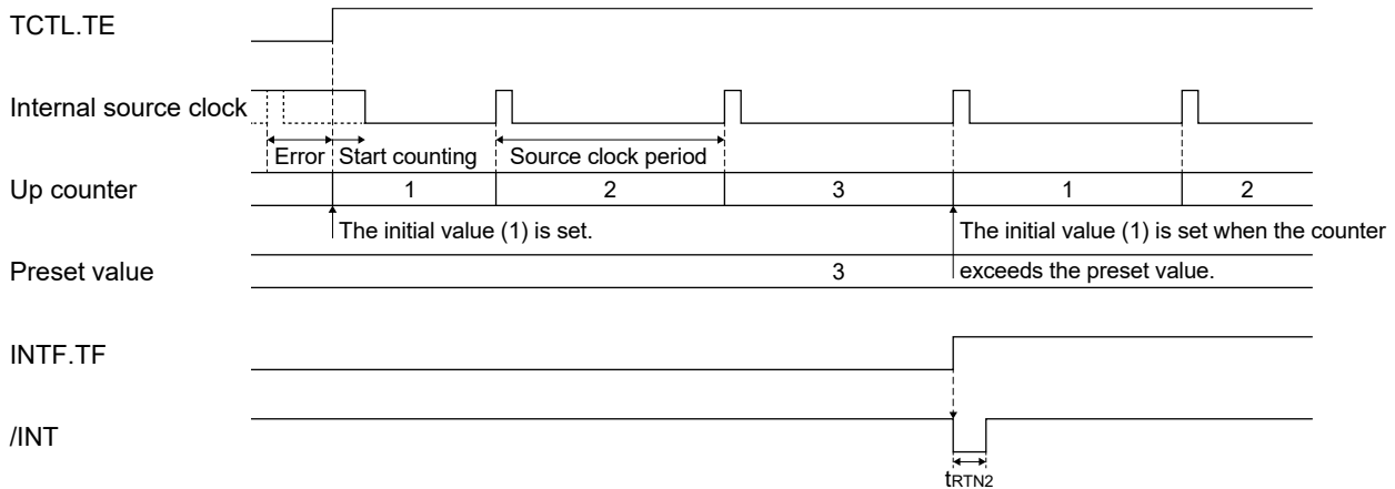
Figure 3.14 Wakeup Timer Count-Up Operation
