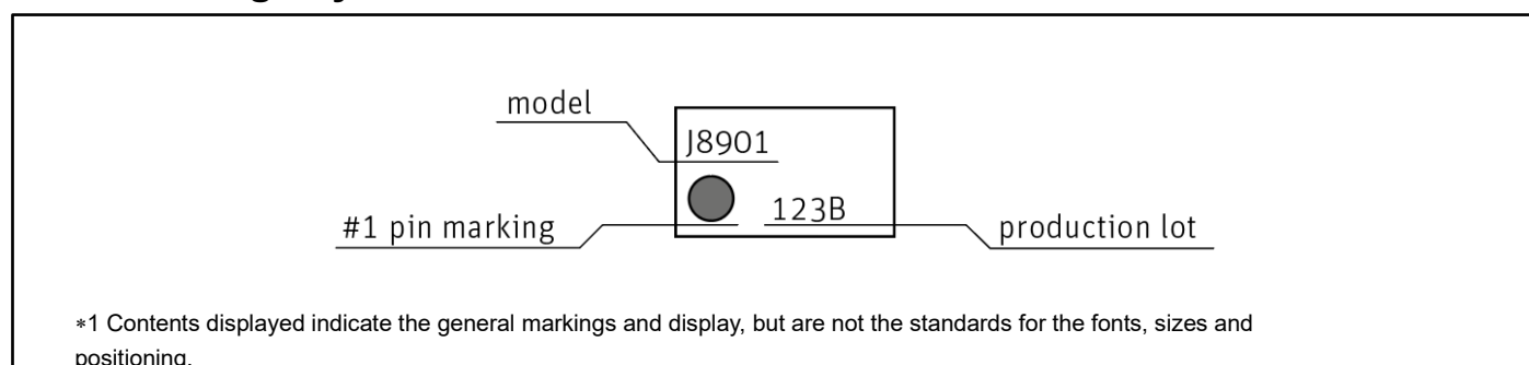
Figure 6.2 Marking Layout
