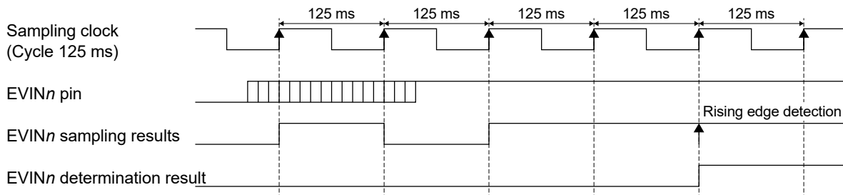
Figure 3.27 EVIN Noise Filter Function
