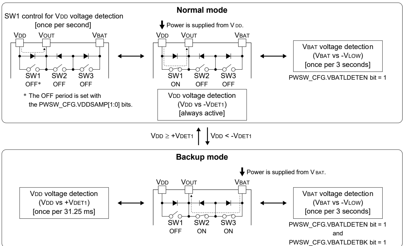
Figure 3.22 Power Switching Control 1 (when using a primary battery as V_{BAT} )
