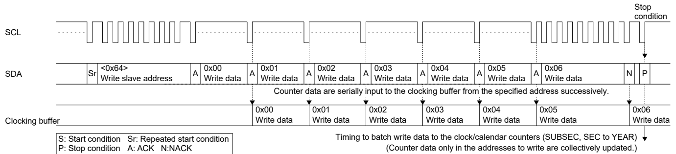
Figure 3.6 I 2 C-Bus Interface Clock/Calendar Counters Access Timing
