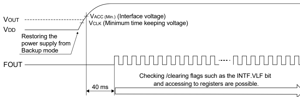
Figure 2.8 Restoring from Backup Mode
