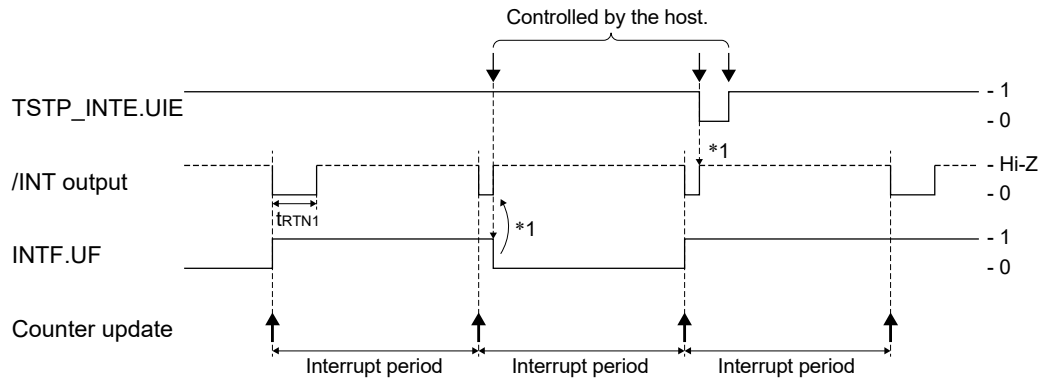
Figure 3.9 Time Update Interrupt Timing Chart
