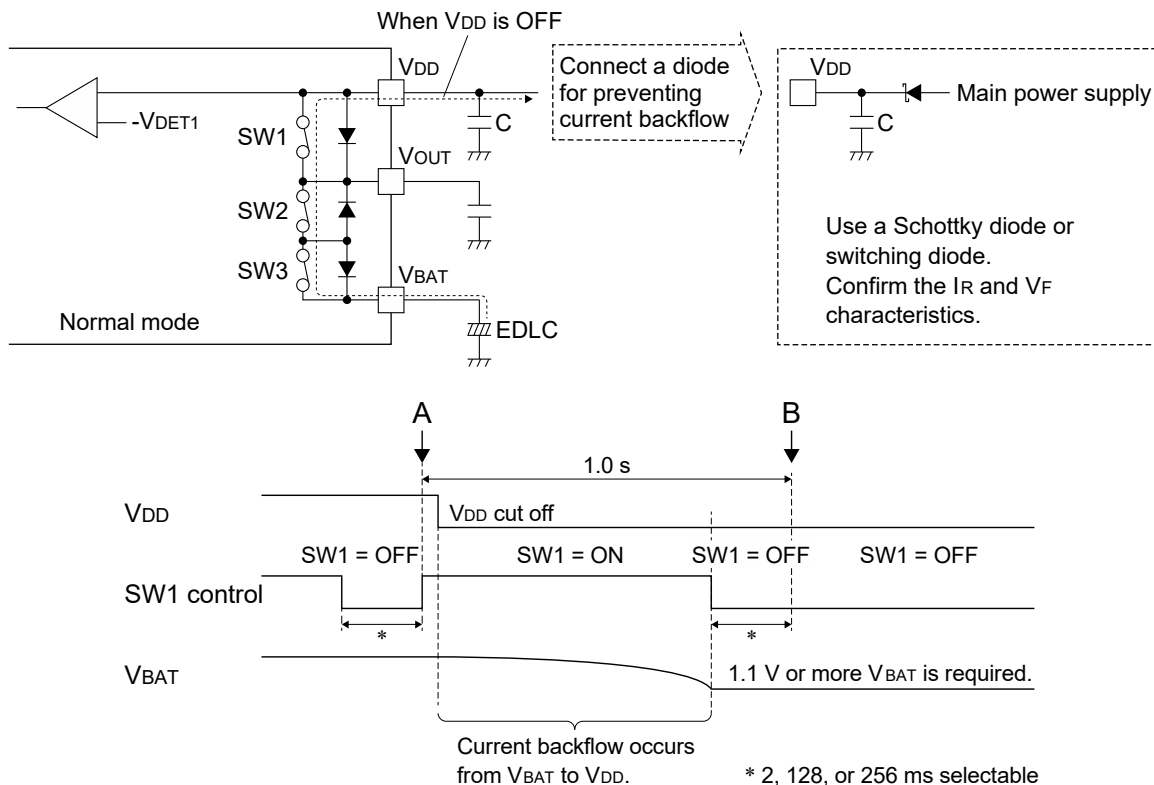
Figure 3.25 Notes on Using Small EDLC
