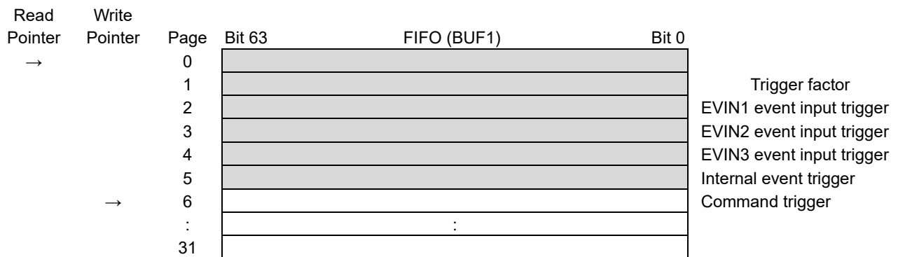
Figure 3.29 Time Stamp Buffer in FIFO Mode (example when six data have been stored)
