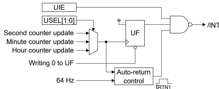
Figure 3.8 Configuration of Time Update Interrupt Circuit
