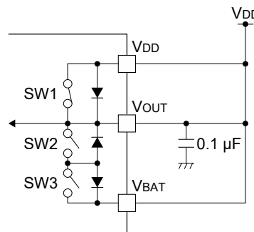
Figure 2.4 Power Supply Connection Example (3)
