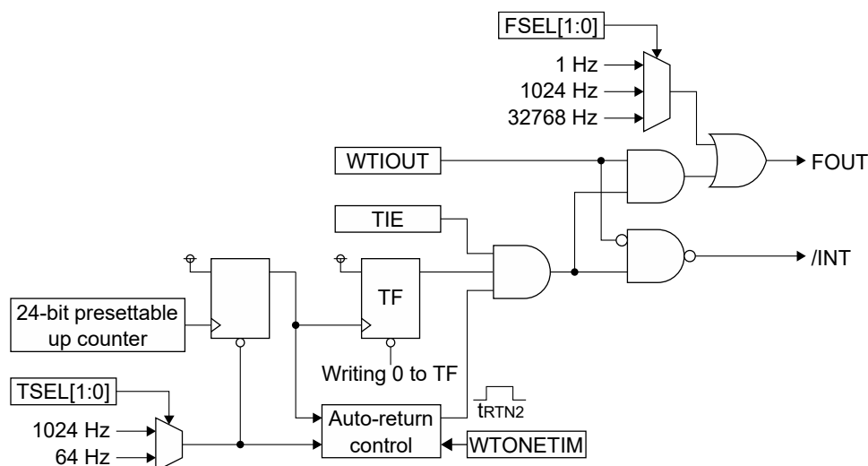
Figure 3.16 Configuration of Wakeup Timer Interrupt Circuit
