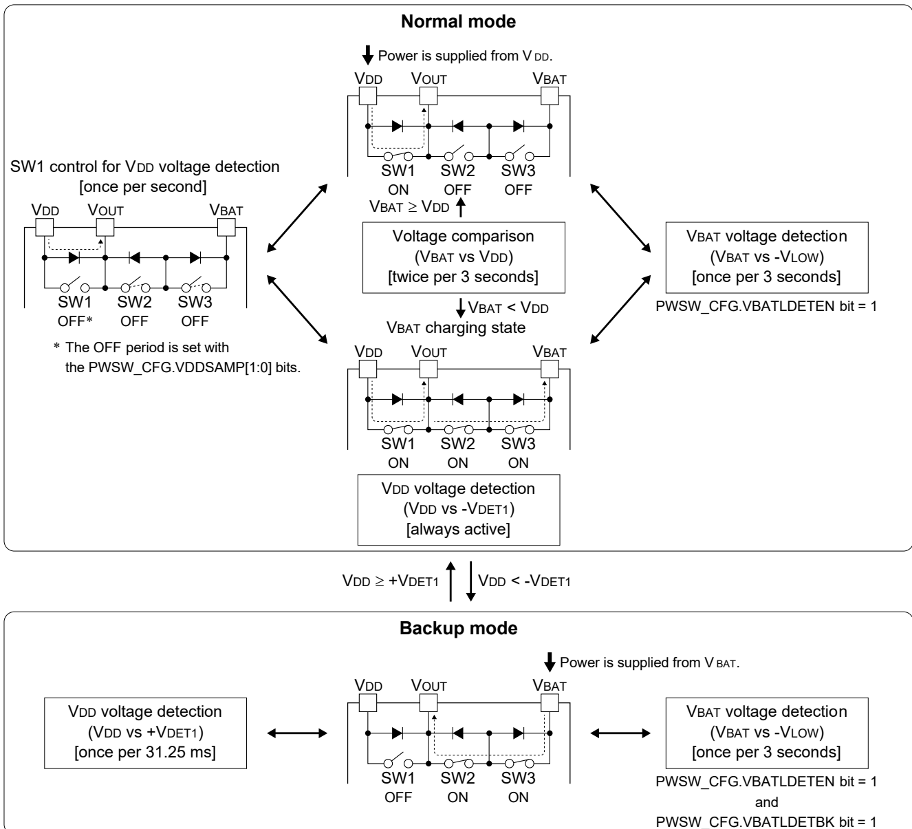
Figure 3.23 Power Switching Control 2 (when using a secondary battery as V_{BAT} )
