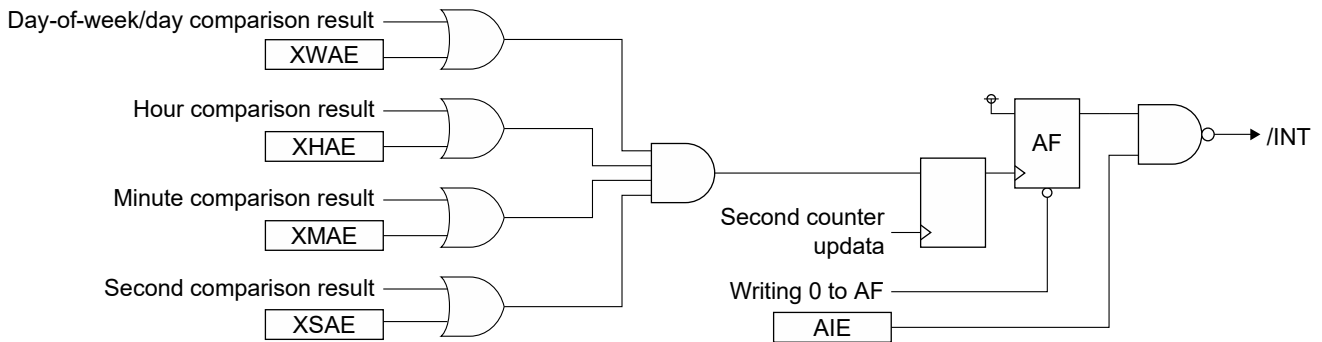
Figure 3.11 Configuration of Alarm Interrupt Circuit
