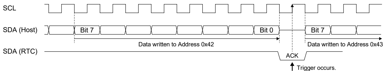
Figure 3.35 Command trigger Timing
