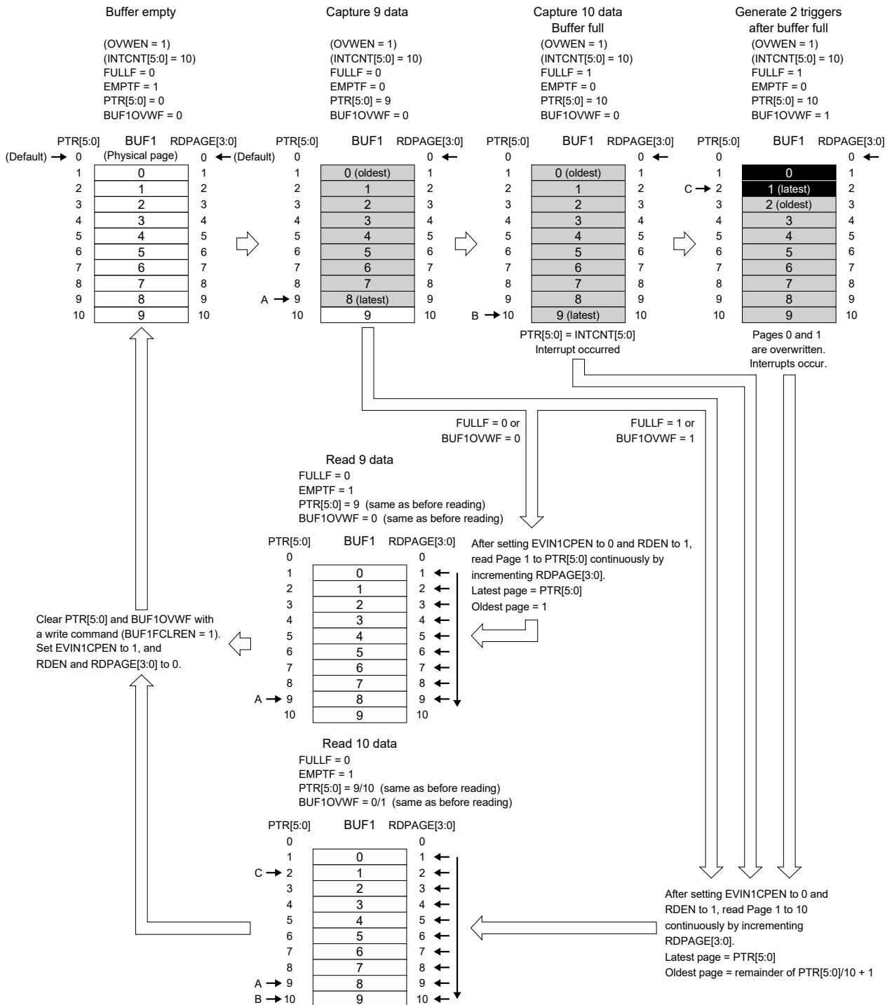
Figure 3.34 Time Stamp Capture Operations (Direct mode + Overwrite mode)
