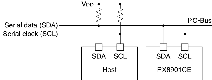
Figure 3.1 Example of Connection Between I 2 C-Bus Host and JR8901-32
