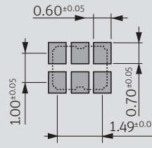
pad layout
