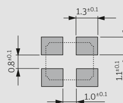
pad layout
