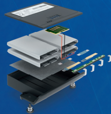
Customized battery packs
