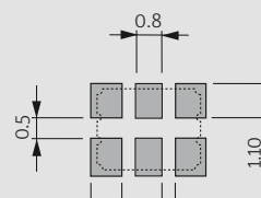
pad layout
