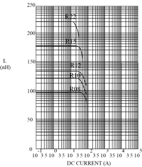
@ INDUCTANCE VS. DC SUPERPOSITION RESPONSE CURVE
