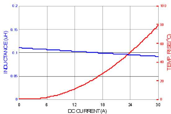
PIC0402HPR10YF
