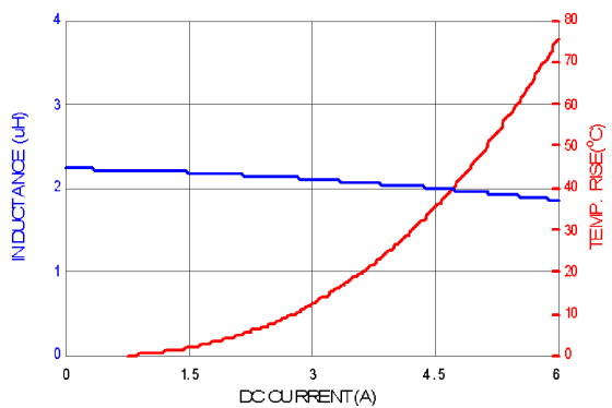
PIC0402HP2R2MF
