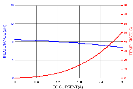
PIC0402HP8R2MF
