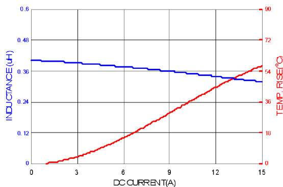
PIC0402HPR36MF
