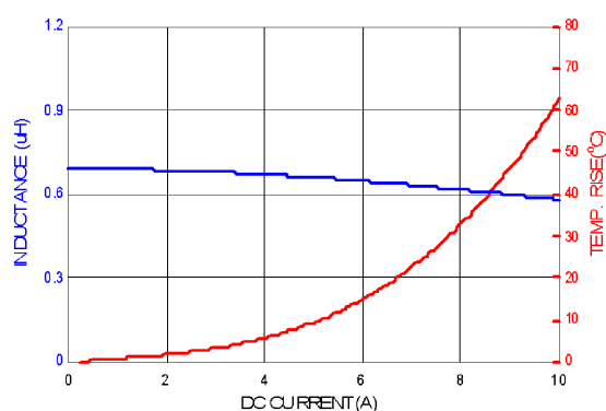
PIC0402HP1R2MF
