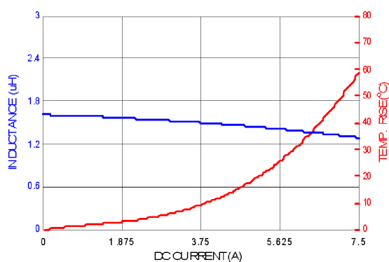
PIC0402HP1R5MF
