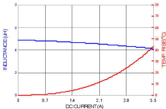
PIC0402HP4R7MF
