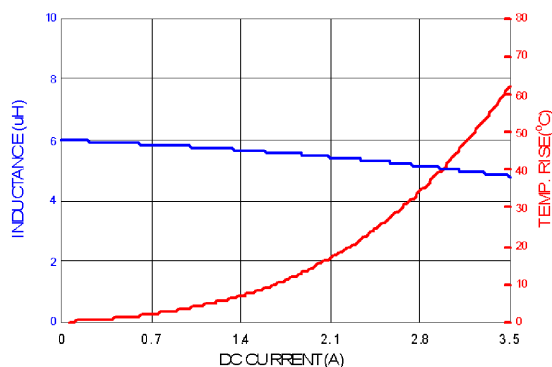
PIC0402HP5R6MF
