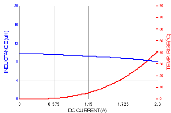
PIC0402HP100MF
