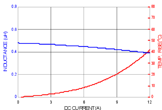
PIC0402HPR47MF
