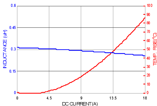
PIC0402HPR47MF
