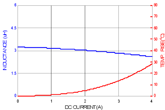
PIC0402HP3R3MF
