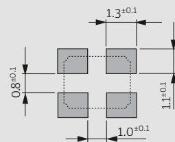
pad layout
